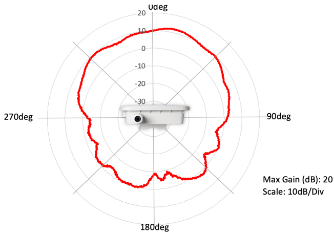
2.4 GHz Azimuth
